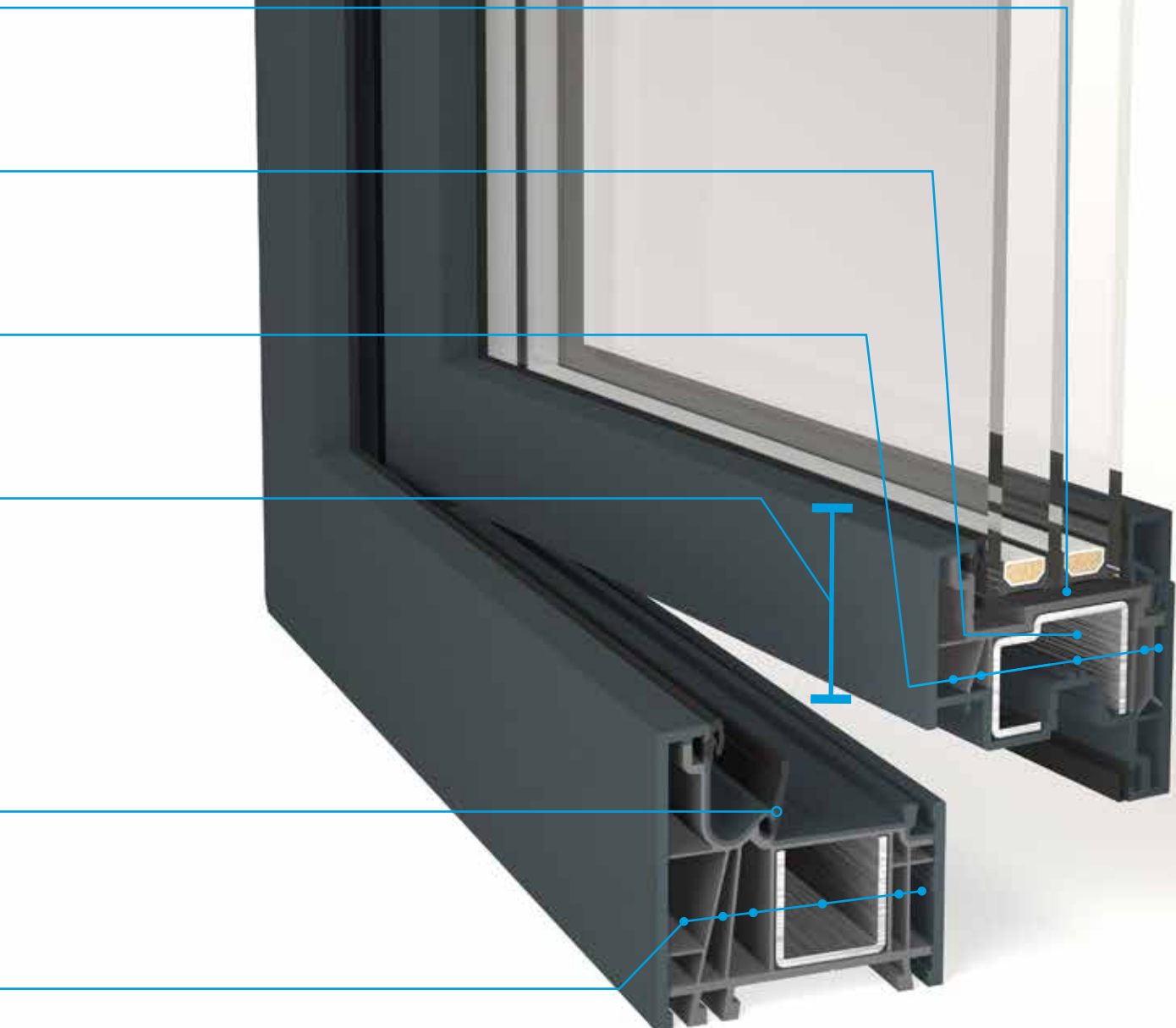
Section 74 mm
